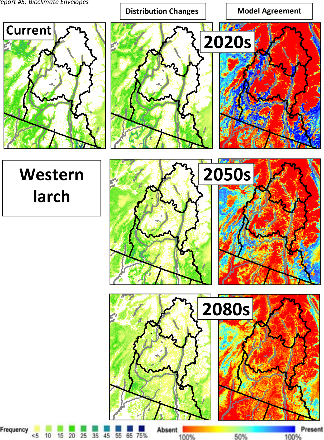
Figure 3.12. Current and projected frequencies for western larch. Future estimates are averages of bioclimate envelope shift projections from 18 climate scenarios. The right column shows the presence/ absence agreement between the 18 projections (Gray and Hamann 2011 unpubl. data).
