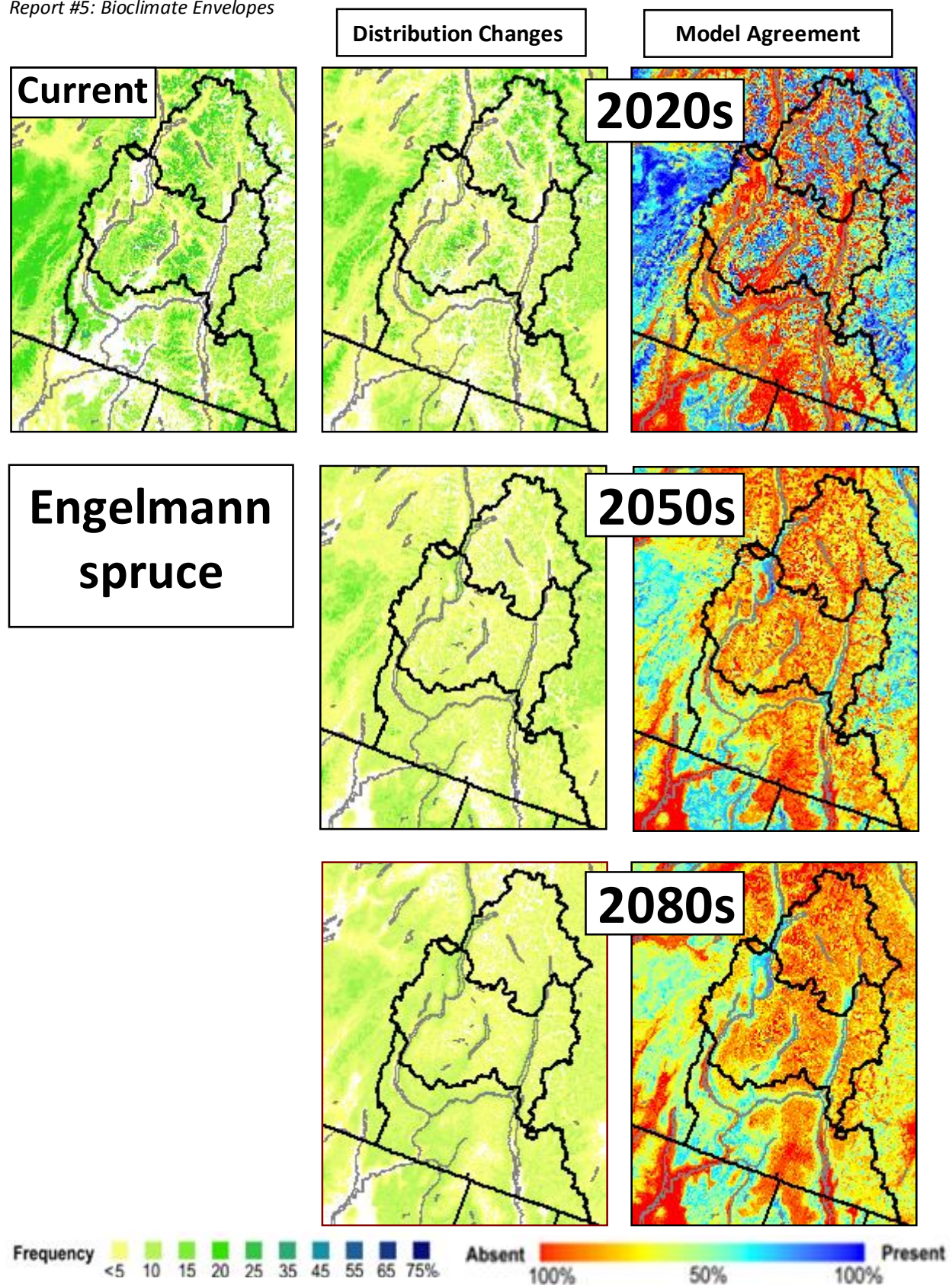
Figure 3.15. Current and projected frequencies for Engelmann spruce. Future estimates are averages of bioclimate envelope shift projections from 18 climate scenarios. The right column shows the presence/ absence agreement between the 18 projections (Gray and Hamann 2011 unpubl. data).
