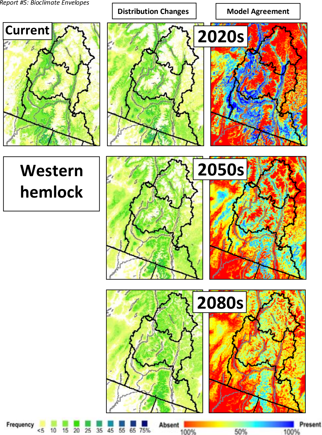
Figure 3.14. Current and projected frequencies for western hemlock. Future estimates are averages of bioclimate envelope shift projections from 18 climate scenarios. The right column shows the presence/ absence agreement between the 18 projections (Gray and Hamann 2011 unpubl. data).
