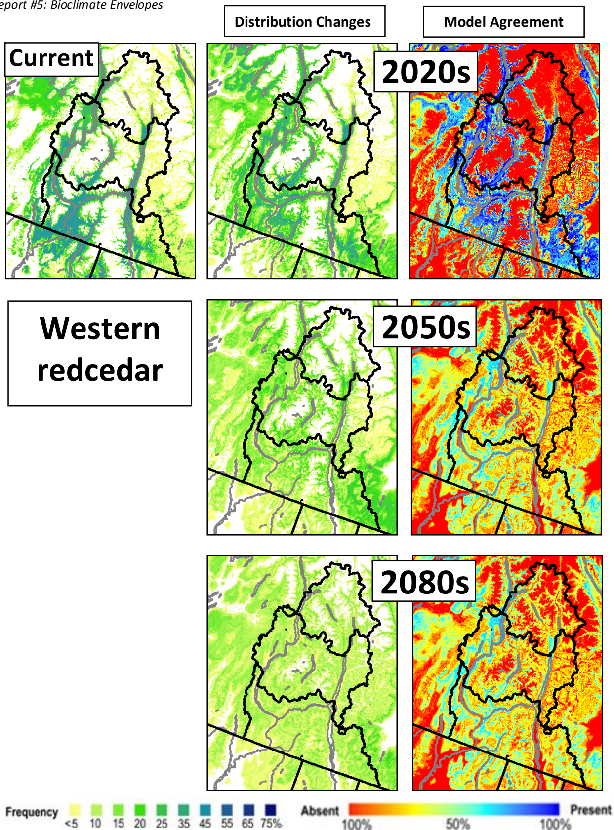
Figure 3.13. Current and projected frequencies for western redcedar. Future estimates are averages of bioclimate envelope shift projections from 18 climate scenarios. The right column shows the presence/ absence agreement between the 18 projections (Gray and Hamann 2011 unpubl. data).
