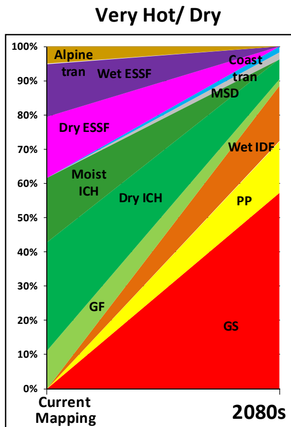
Figure 3.8. Schematic representations of projected bioclimate envelope shifts for the South subregion under three climate scenarios.
