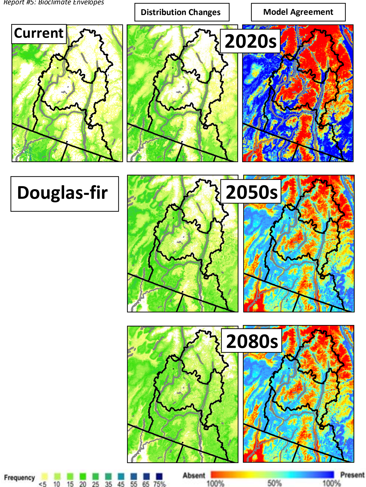
Figure 3.11. Current and projected frequencies for Douglas-fir. Future estimates are averages of bioclimate envelope shift projections from 18 climate scenarios. The right column shows the presence/ absence agreement between the 18 projections (Gray and Hamann 2011 unpubl. data).
