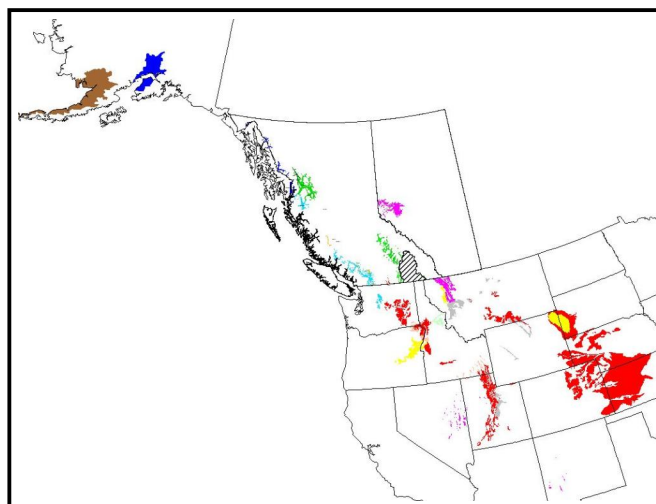
Figure 3.4. Reference period (1961-90) locations of bioclimate envelopes that may occur in the study area in the 2080s based on results from Random-Forest analysis of three climate scenarios. Colours of source areas are consistent with the other figure legends.
